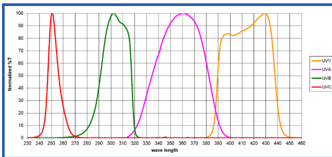
EIT Mercury (Broadband) Responses: UVC, UVB, UVA, UVV
