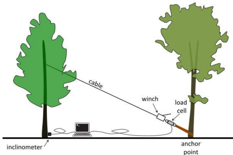
Pulling Test setup for trunk evaluation
