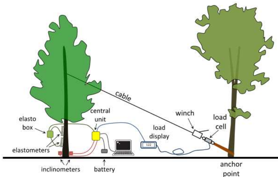
The setup for Pulling Test for both root and trunk evaluation.
