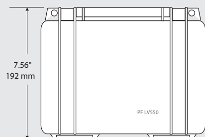
ELECTRONICS ENCLOSURE
