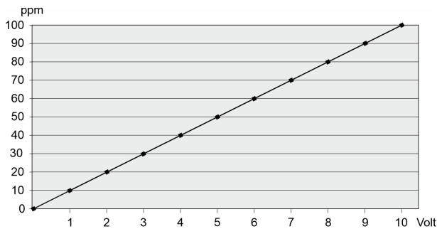
Figure 1: Operation curve.
